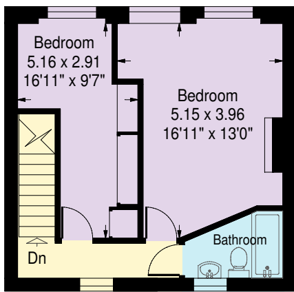
First Floor (Mews house)
